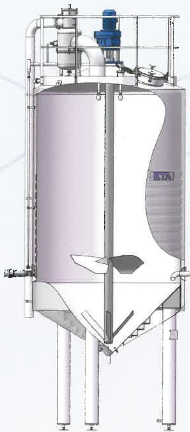
15,000l ultra clean tank Storage of yoghurt Pressure: 0.49 bar
