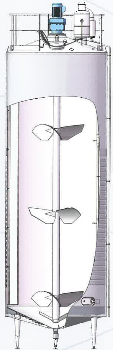
60,000l ultra clean tank Ripening of soft cheese Pressure: 0.1 bar
