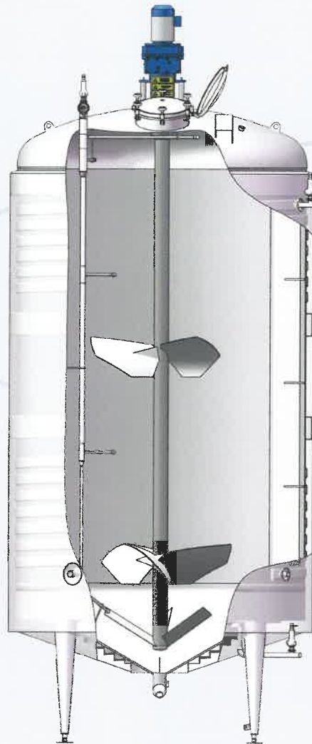
30,000l sterile tank Storage of béchamel Pressure: +4 bar - 1 bar
